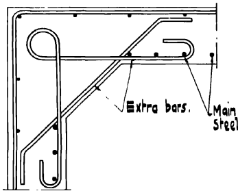
Fig. 248. —Plan of Corner showing Extra Steel required.
